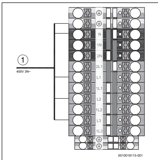
Fig. 47 Spenningsforsyning i leveringstilstand (6 kW, 8 kW, 12 kW, 16 kW)
