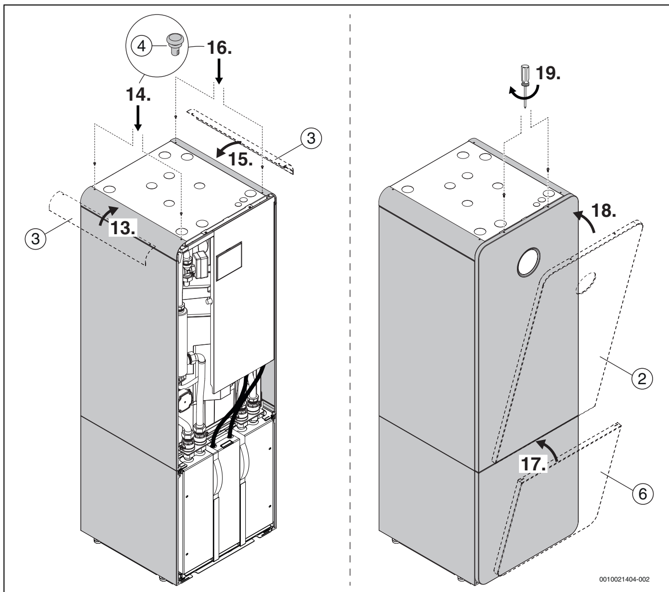
Fig. 23 Designsettmontering
