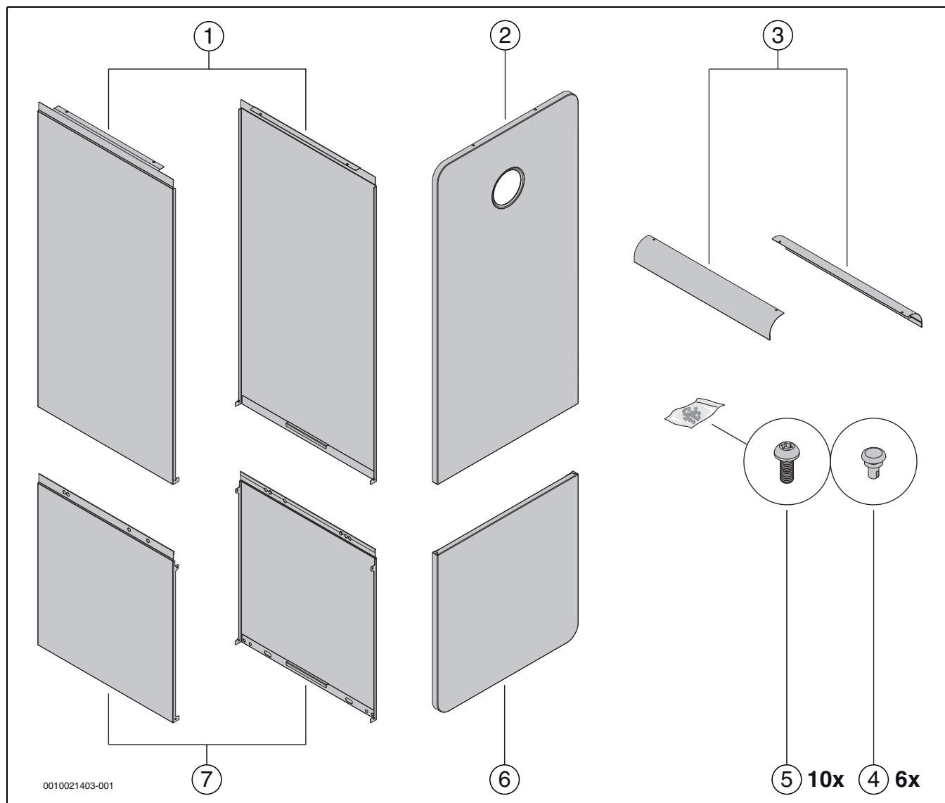
Fig. 21 Designsettmontering
