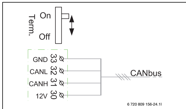
Fig. 18 Terminering CAN-BUS
